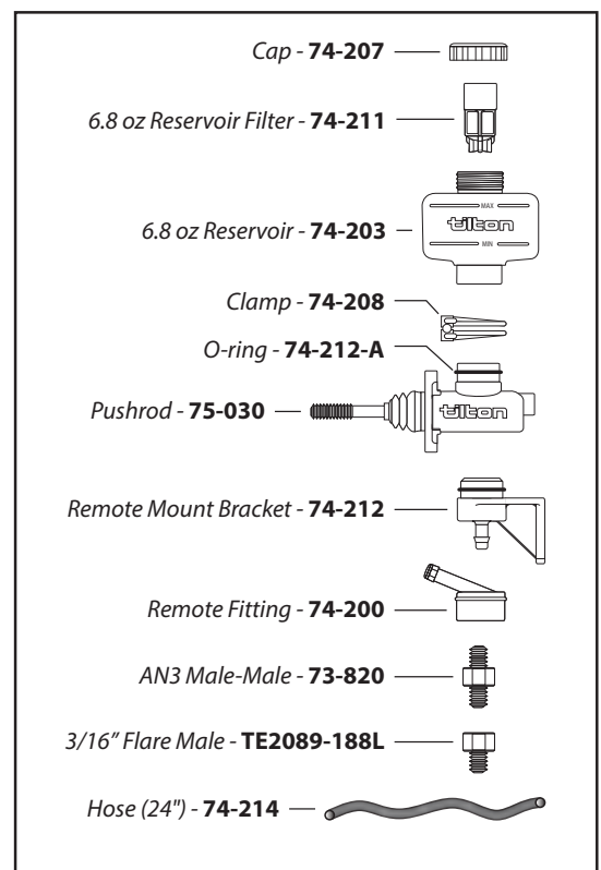
Diagram 1 - Master Cylinder Kit and Replacement Parts
