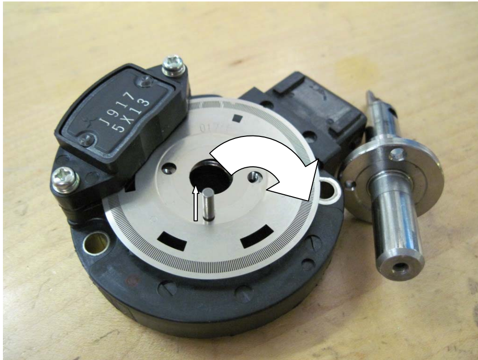
Figure 31: CAS disc screws and shaft removed
