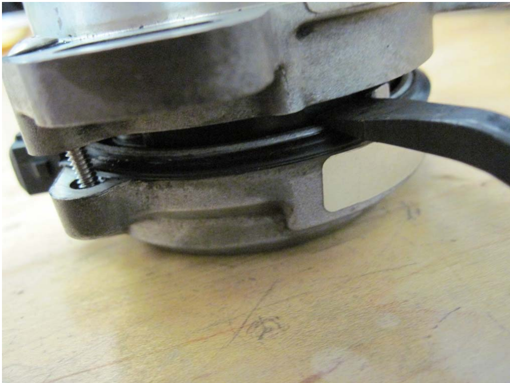
Figure 17: Using prybar to remove cover
