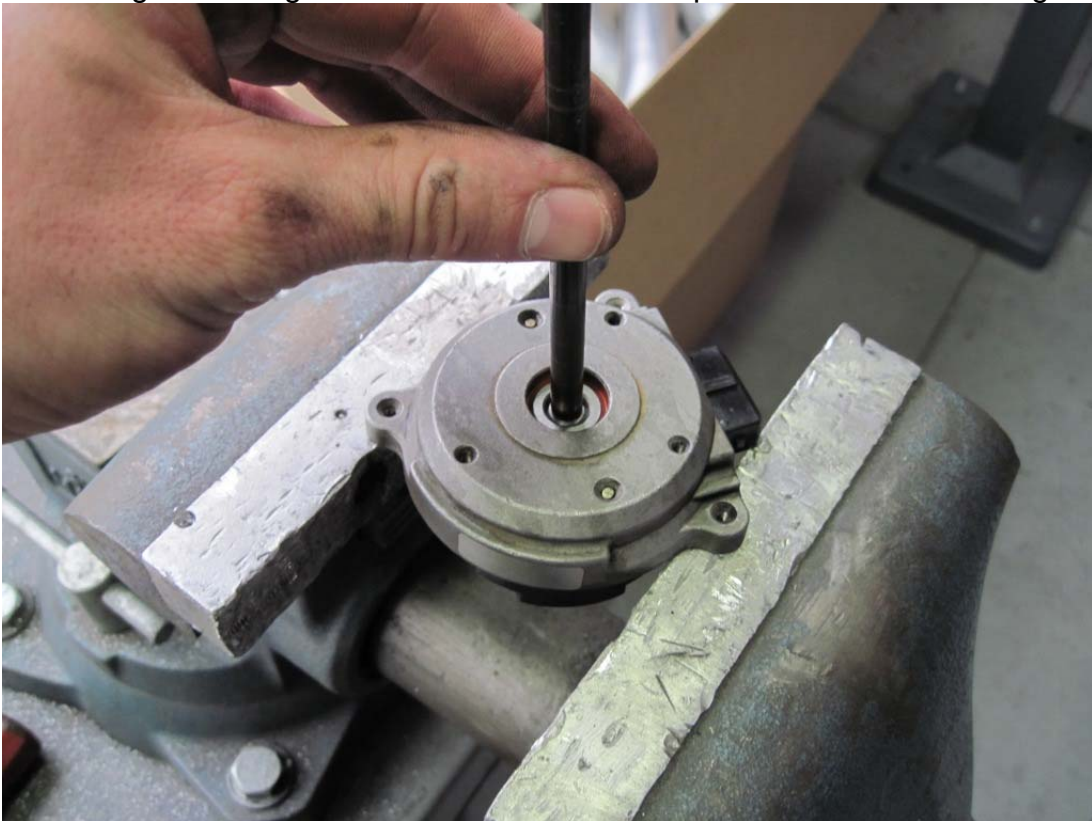
Figure 23: Separation of shaft from housing using 3/8" pin punch and hammer
