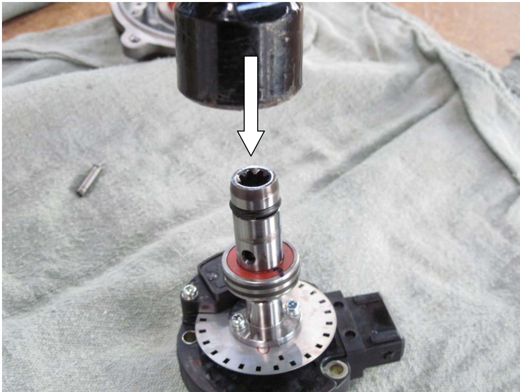
Figure 37: Hammering star socket to press on socket and bearing
