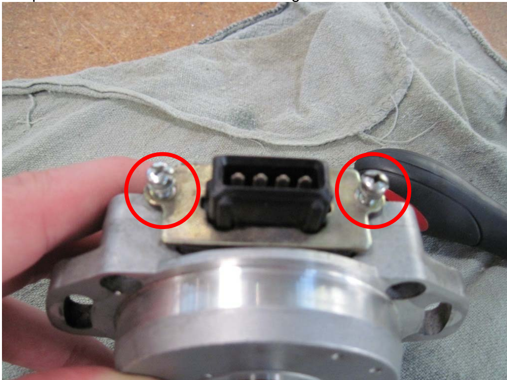
Figure 42: Connector cover reinstalled
