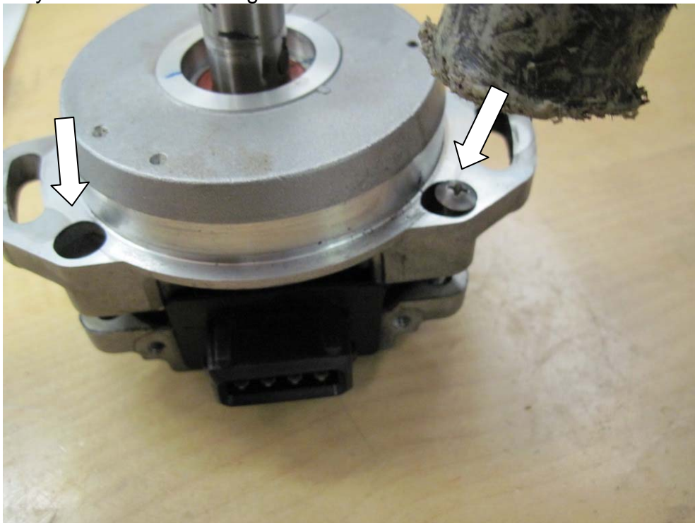
Figure 16: Using cap screws and mallet to loosen/remove cover
