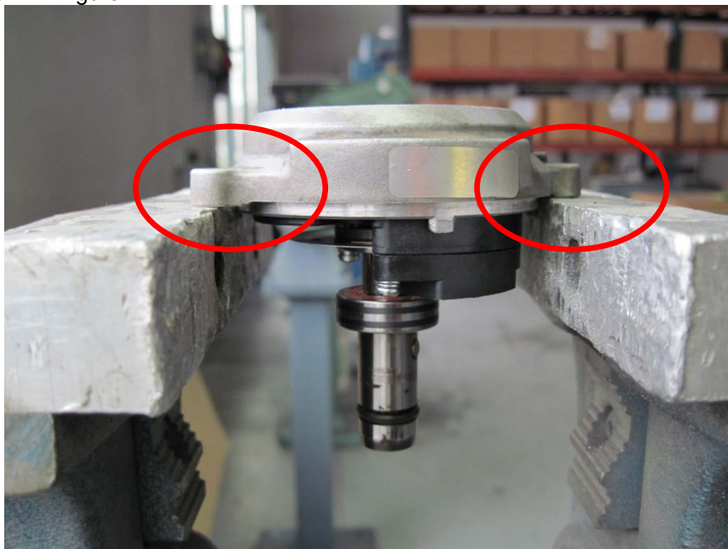
Figure 21: Mounting CAS assembly in vise to separate from shaft
