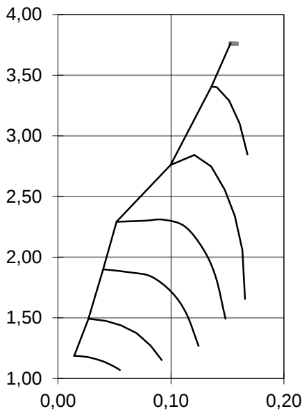
Original compressor
