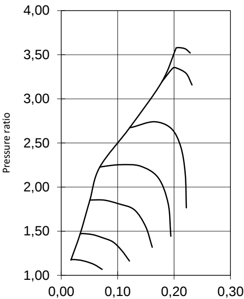
Upgrade compressor
